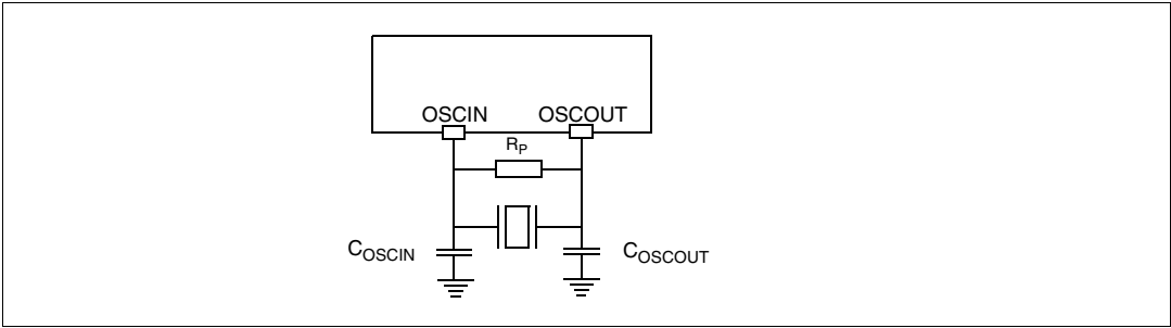
Figure 17. Crystal/ceramic resonator
