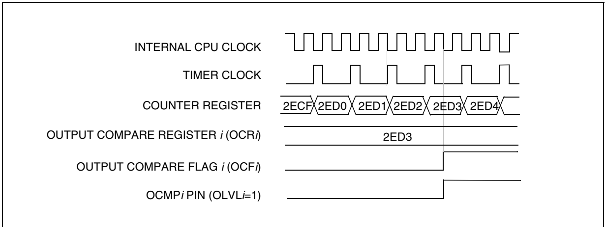
Figure 46. Output Compare Timing Diagram, f_{TIMER} = f_{CPU}/2
