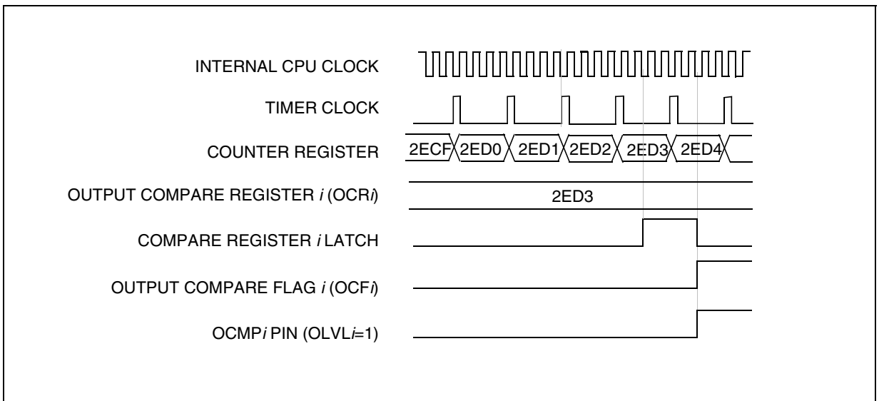
Figure 47. Output Compare Timing Diagram, f_{TIMER} = f_{CPU}/4
