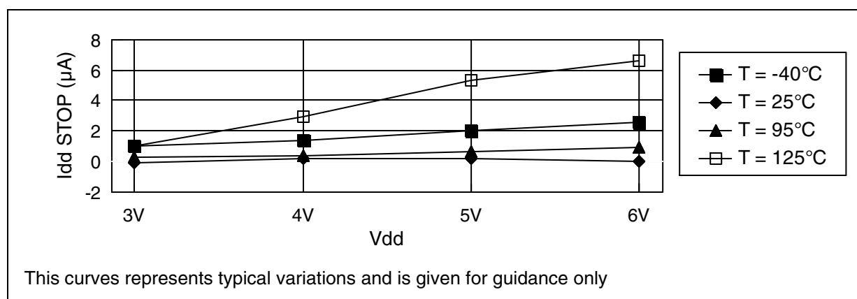
Figure 43. Idd STOP versus VDD for OTP devices
