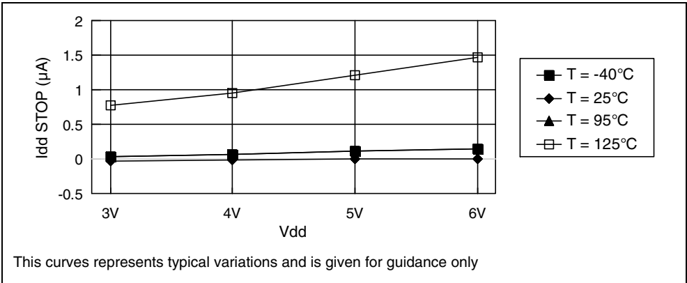
Figure 45. Idd STOP versus VDD for ROM devices
