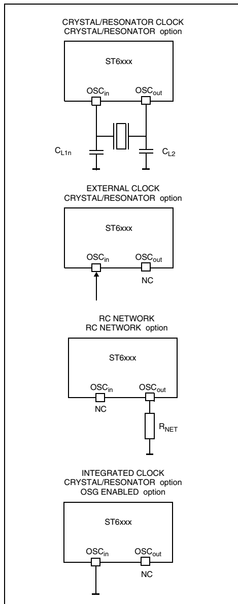
Figure 9. Oscillator Configurations
