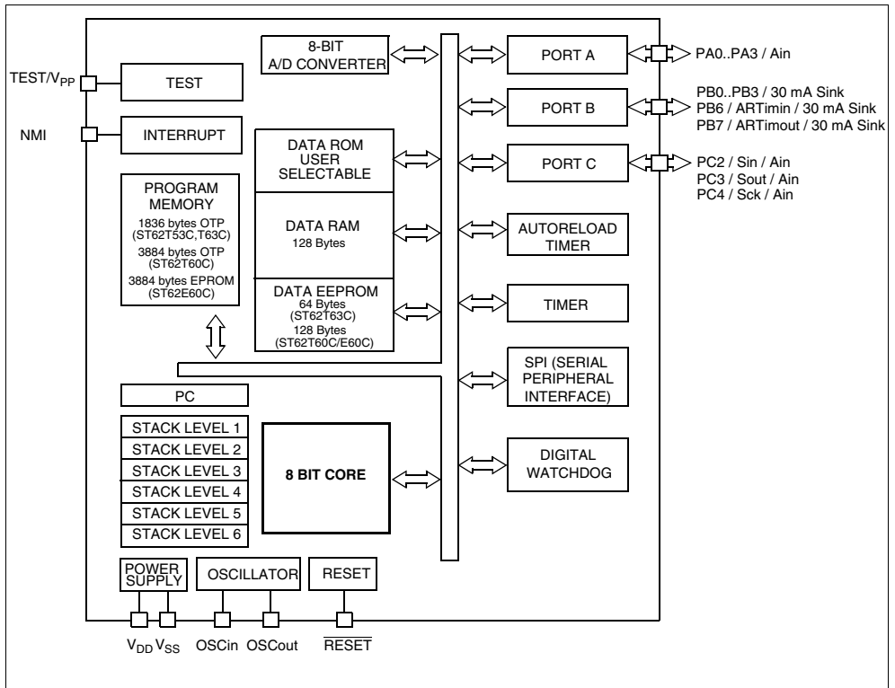
Figure 1. Block Diagram
