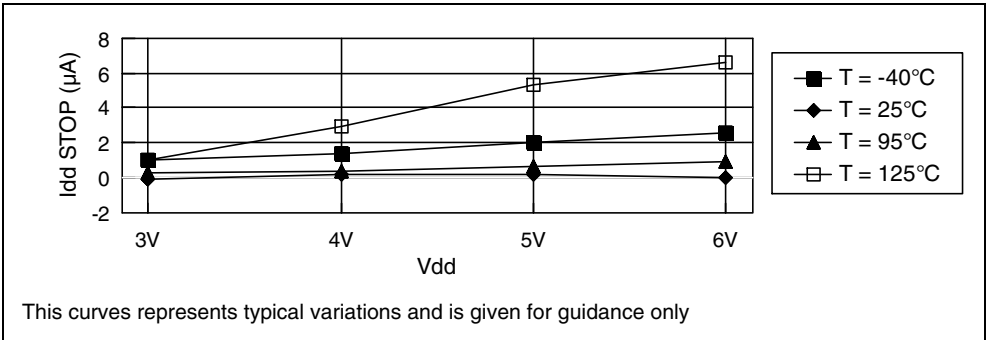
Figure 45. Idd STOP versus VDD for ROM devices
