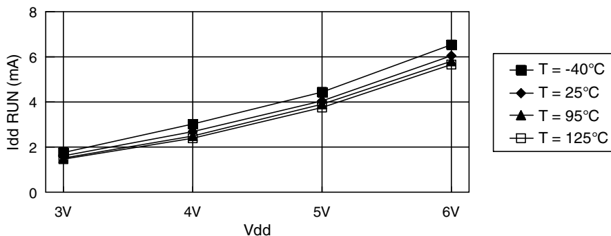
Figure 47. Idd RUN versus V_{DD} at 8 Mhz for ROM and OTP devices
