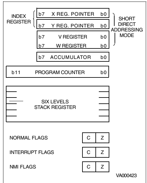
Figure 8. ST6 CPU Programming Mode
