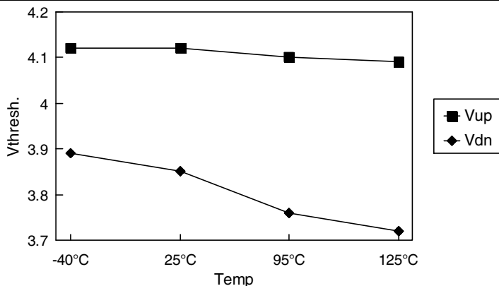
Figure 48. LVD thresholds versus temperature
