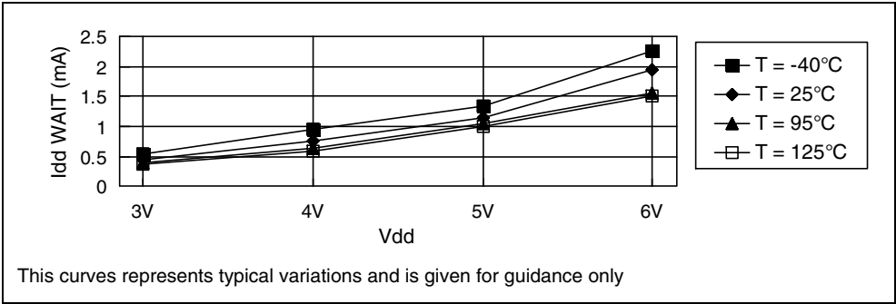
Figure 44. Idd STOP versus VDD for OTP devices
