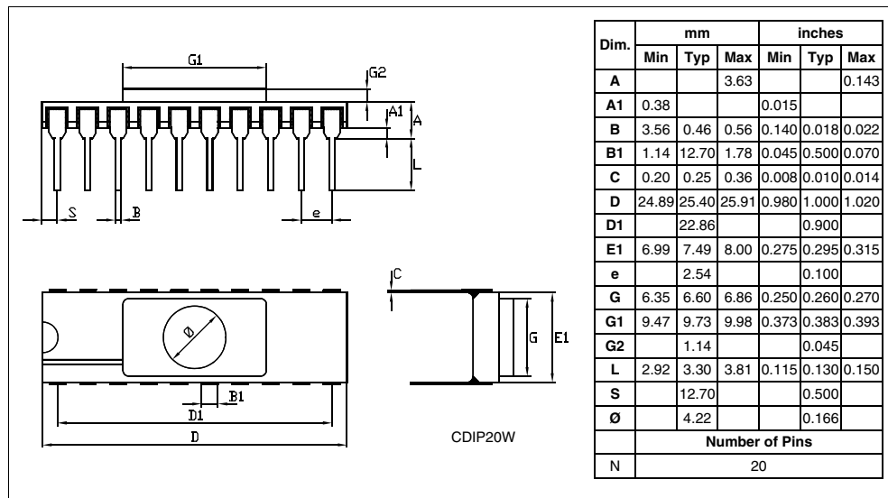
Figure 52. 20-Pin Ceramic Side-Brazed Dual In-Line Package
