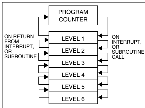
Figure 8. Stack manipulation
