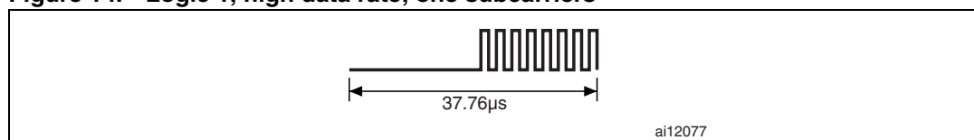
Figure 14. Logic 1, high data rate, one subcarriers
