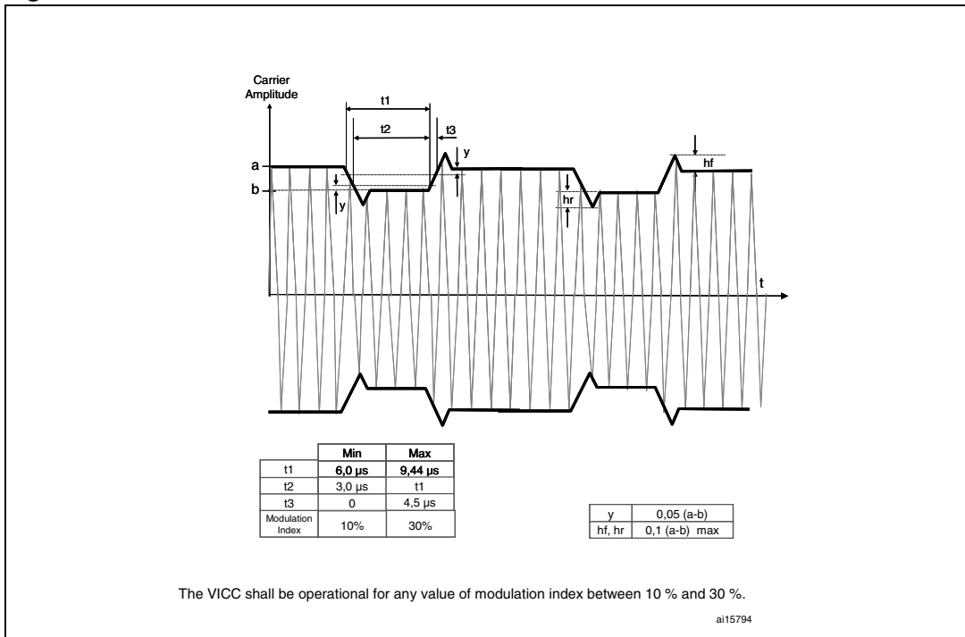
Figure 4. 10% modulation waveform
