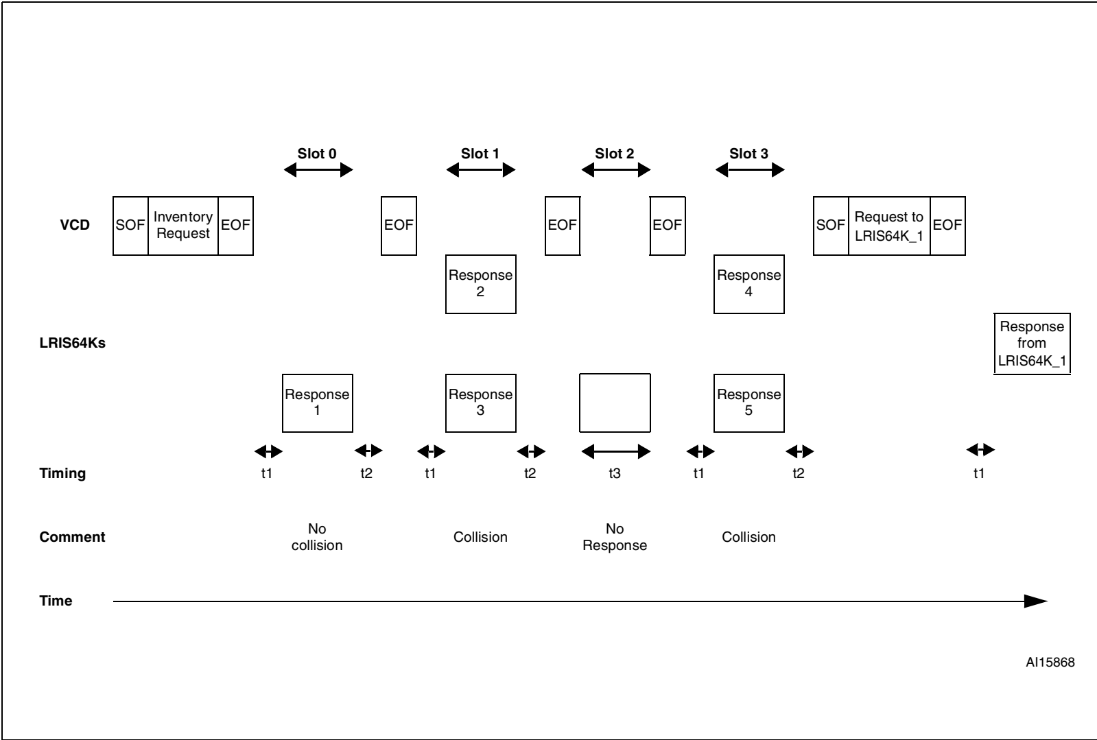
Figure 40. Description of a possible anticollision sequence
