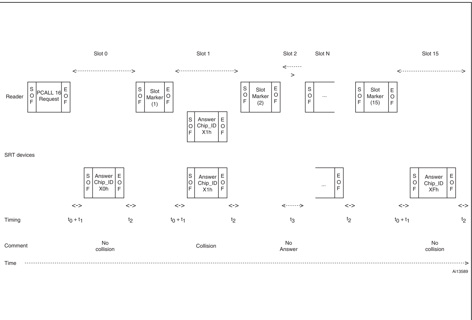
Figure 20. Description of a possible anticollision sequence
