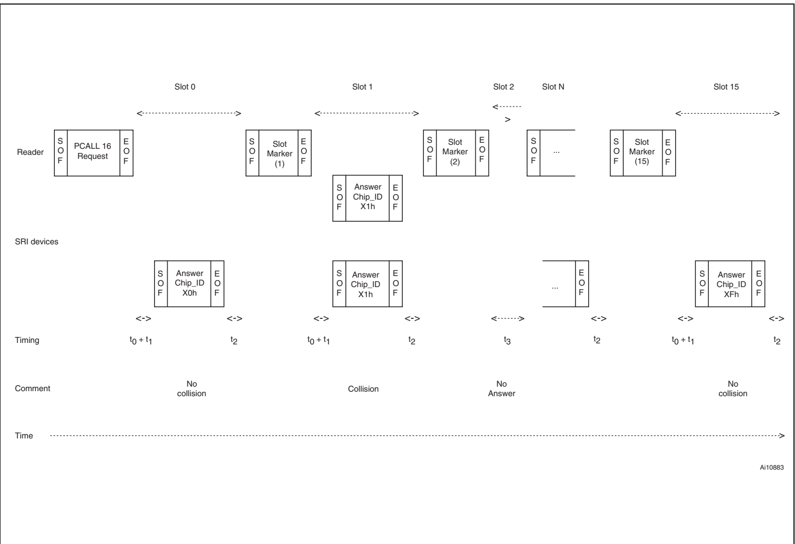
Figure 21. Description of a possible anticollision sequence
