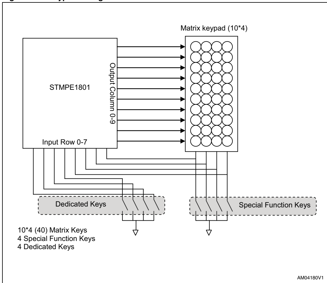
Figure 9. Keypad configurations
