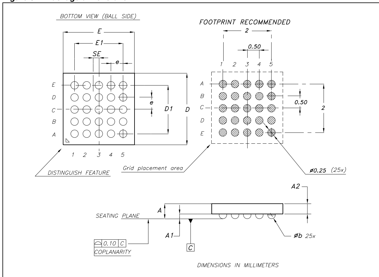
Figure 6. Package dimensions
