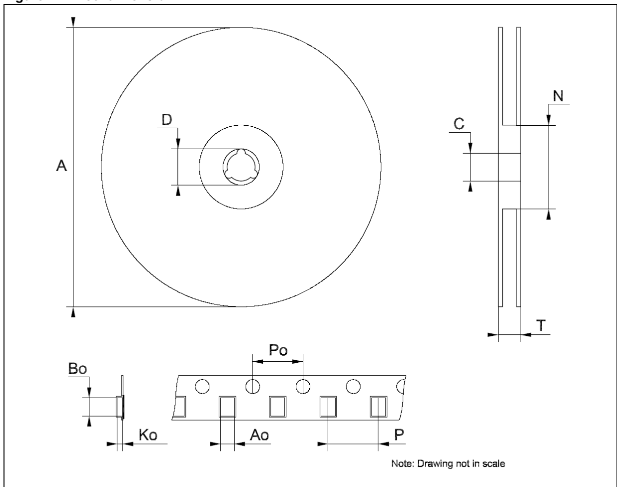
Figure 7. Reel dimension
