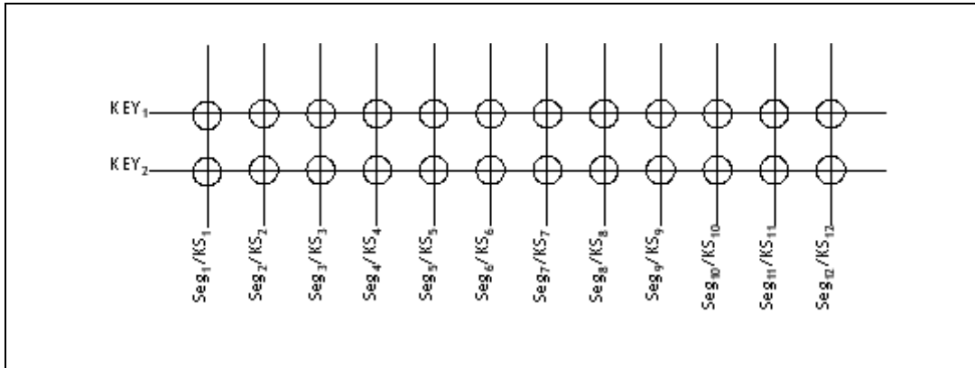
Figure 11. Key storage and READ access
