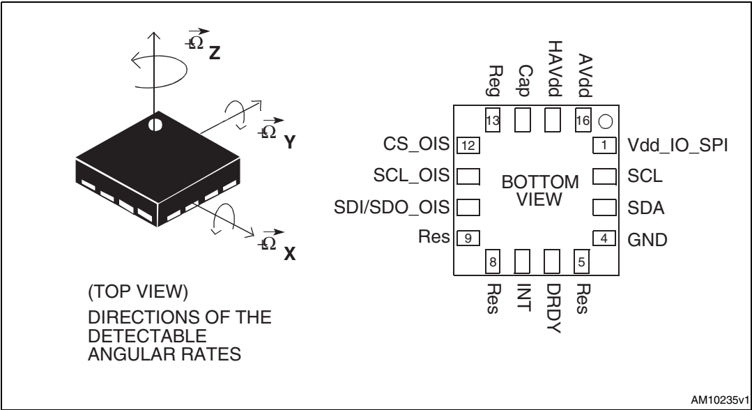
Figure 2. Pin connection
