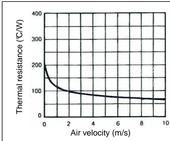
Figure 8. Thermal resistance junction to air
