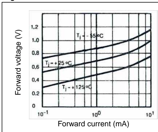
Figure 12. Forward characteristics
