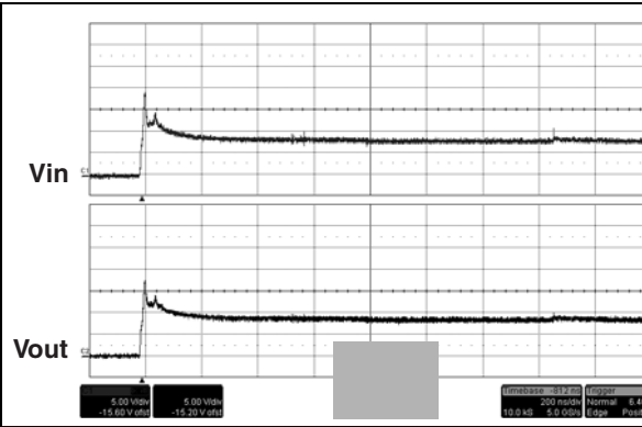
Figure 7. ESD response to ISO10605, C = 150 pF, R = 330 \Omega (+15 kV air discharge)
