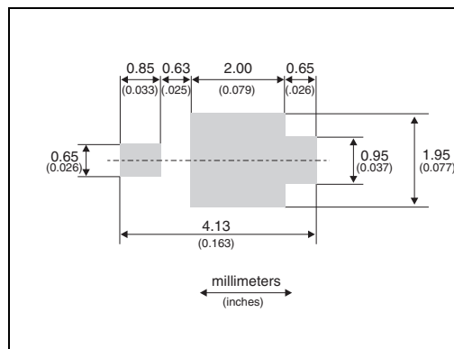
Figure 9. STmite flat footprint dimensions
