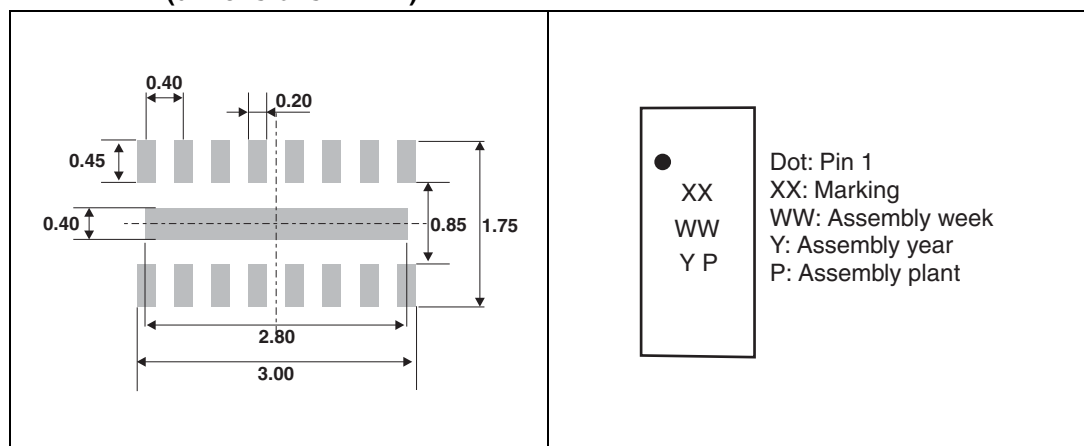
Figure 9. Footprint recommendations (dimensions in mm)
