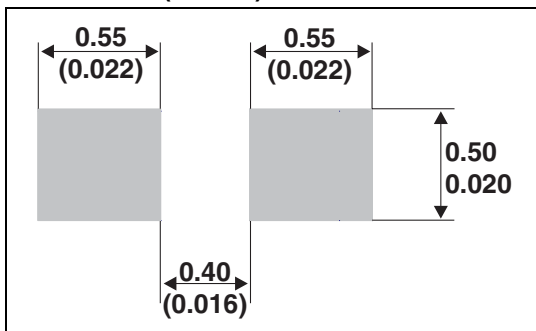
Figure 21. SOD882T footprint in mm (inches)
