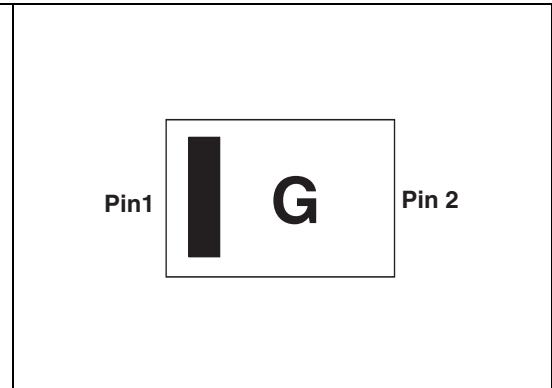
Figure 18. SOD882 marking
