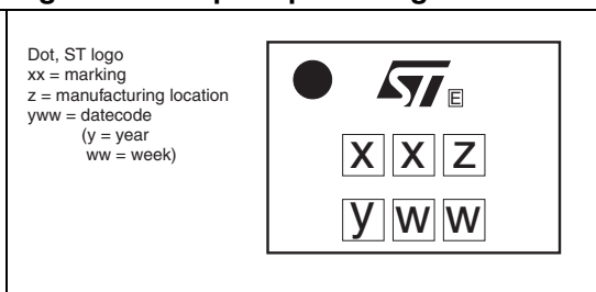
Figure 27. Flip-Chip marking
