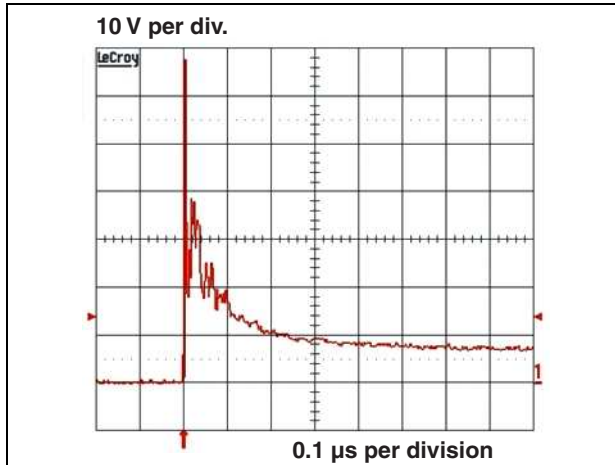
Figure 13. Digital crosstalk test measurement
