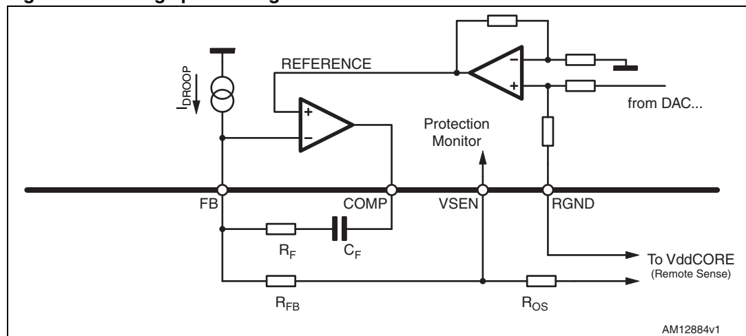
Figure 10. Voltage positioning
