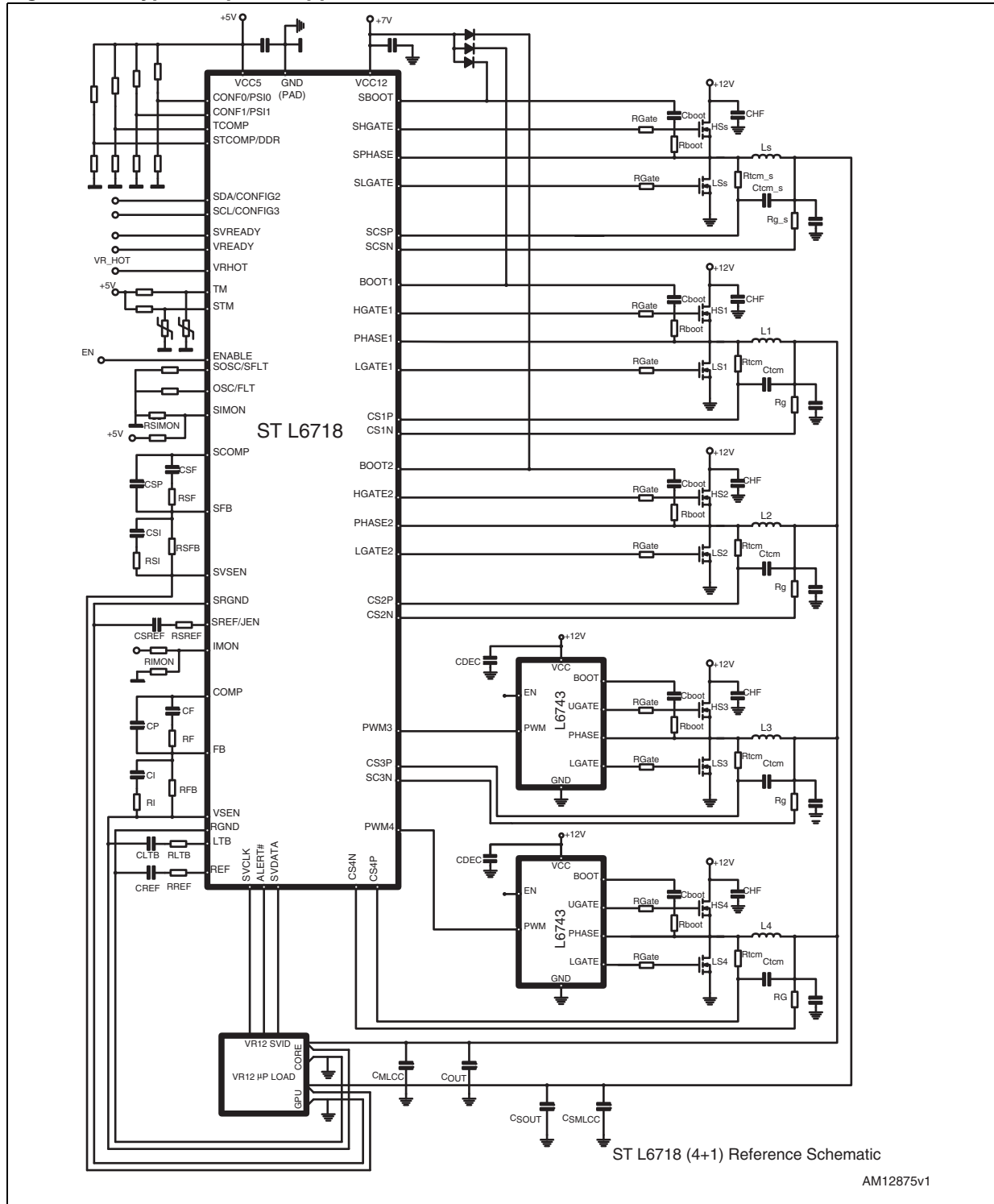
Figure 1. Typical 4-phase application circuit
