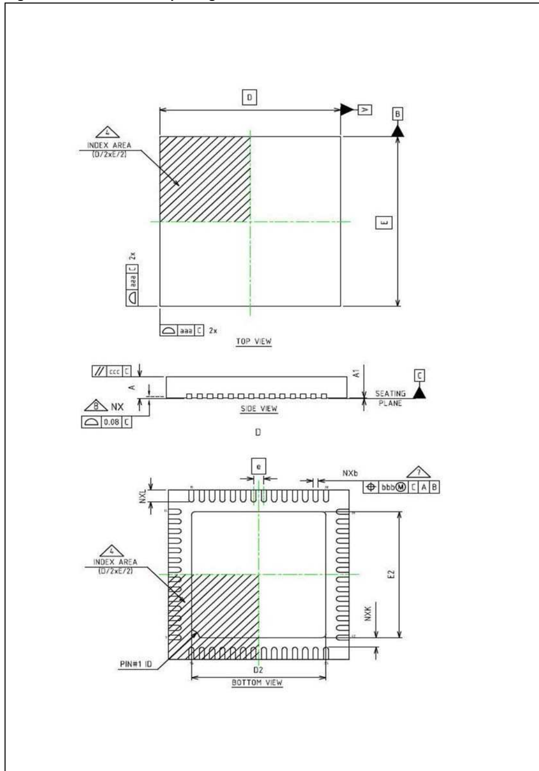
Figure 17. VFQFPN56 7x7 package dimensions
