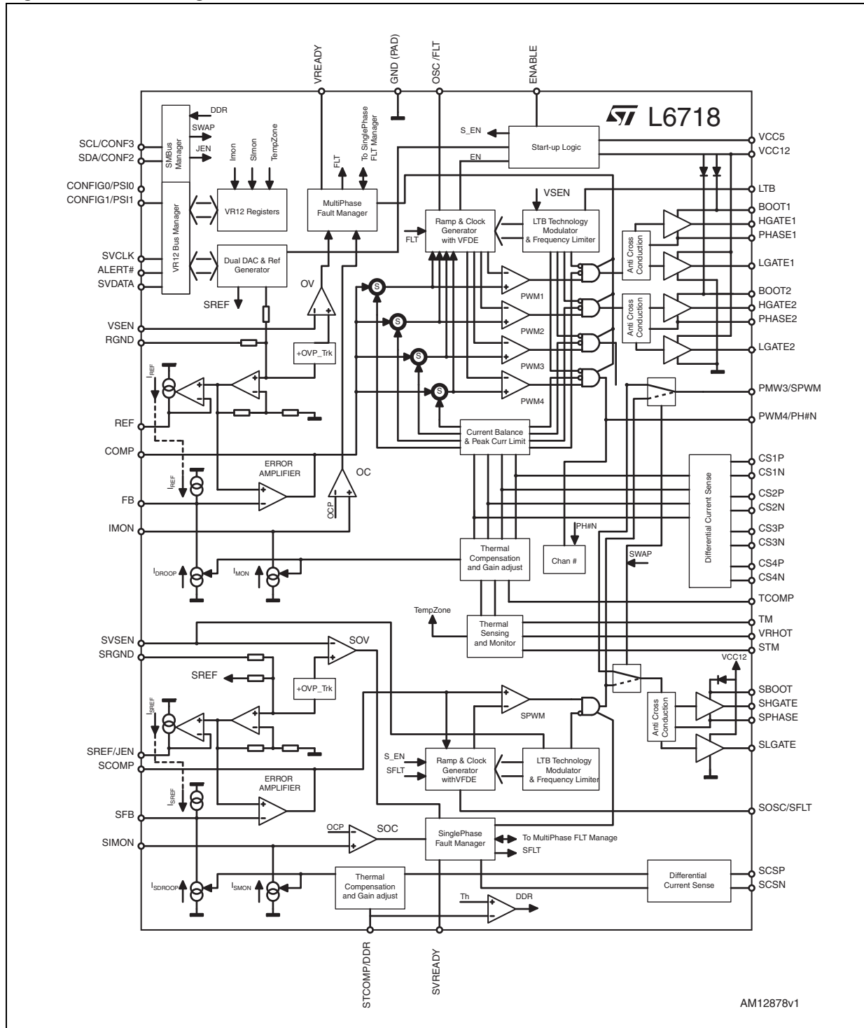
Figure 4. Block diagram
