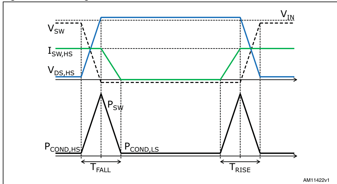
Figure 8. Switching losses
