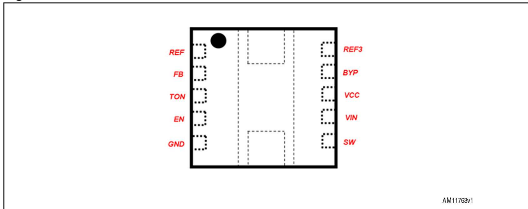
Figure 3. Pinout
