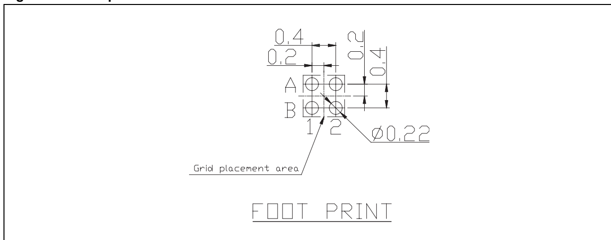
Figure 23. Footprint data
