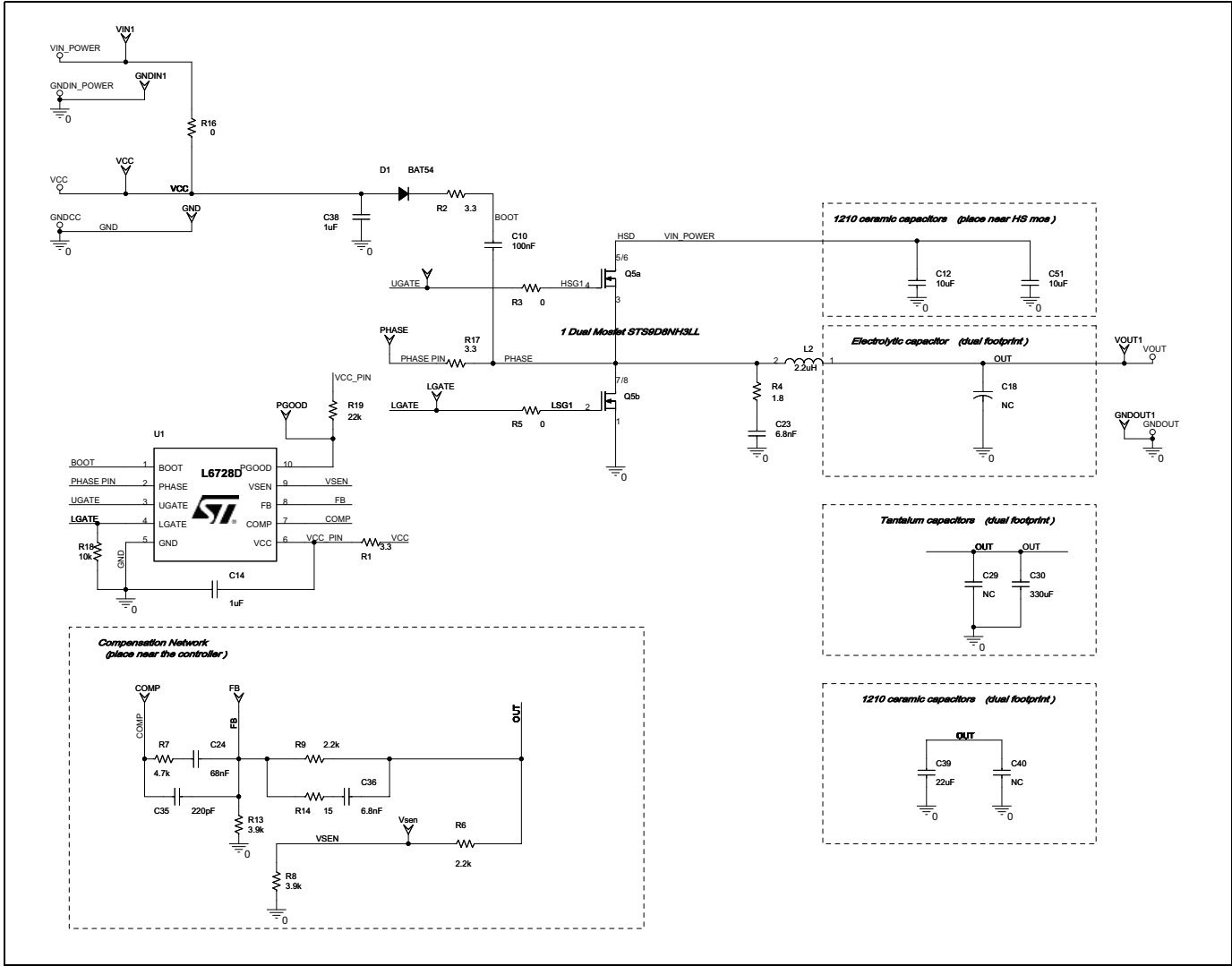
Figure 17. 5 A demonstration board schematic
