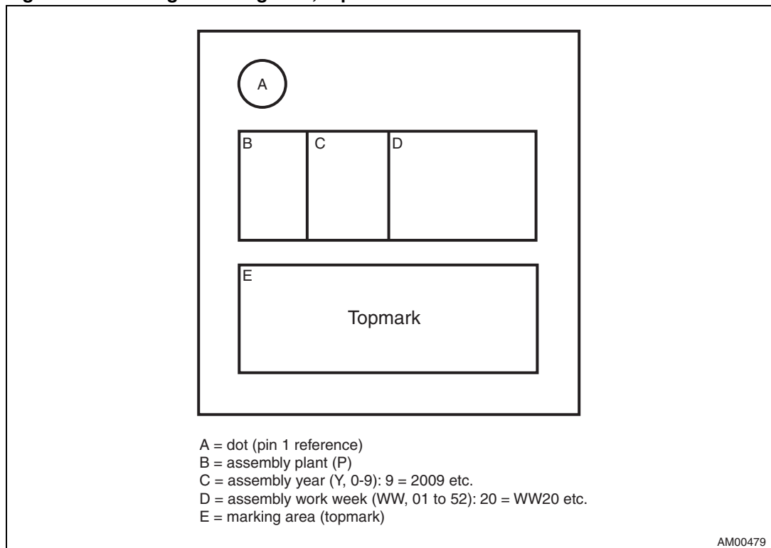
Figure 17. Package marking area, top view
