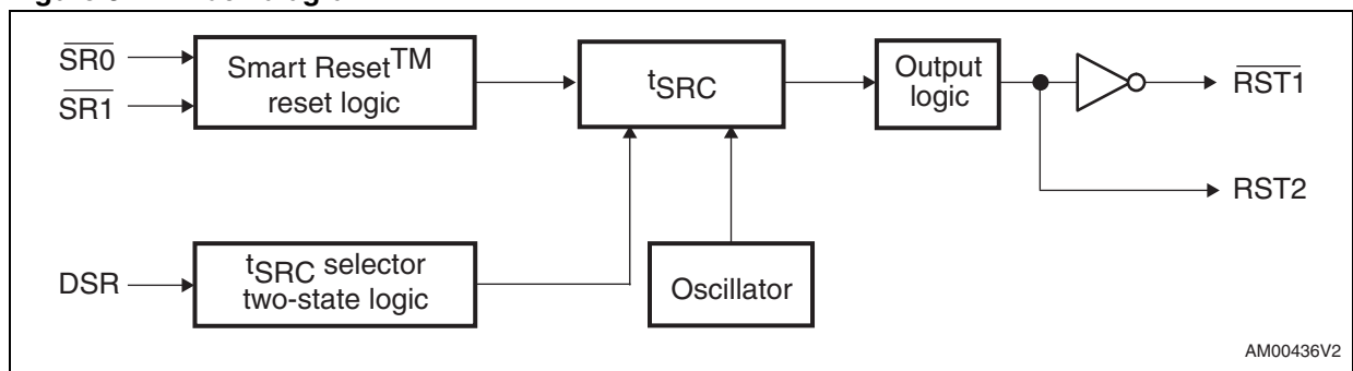
Figure 3. Block diagram
