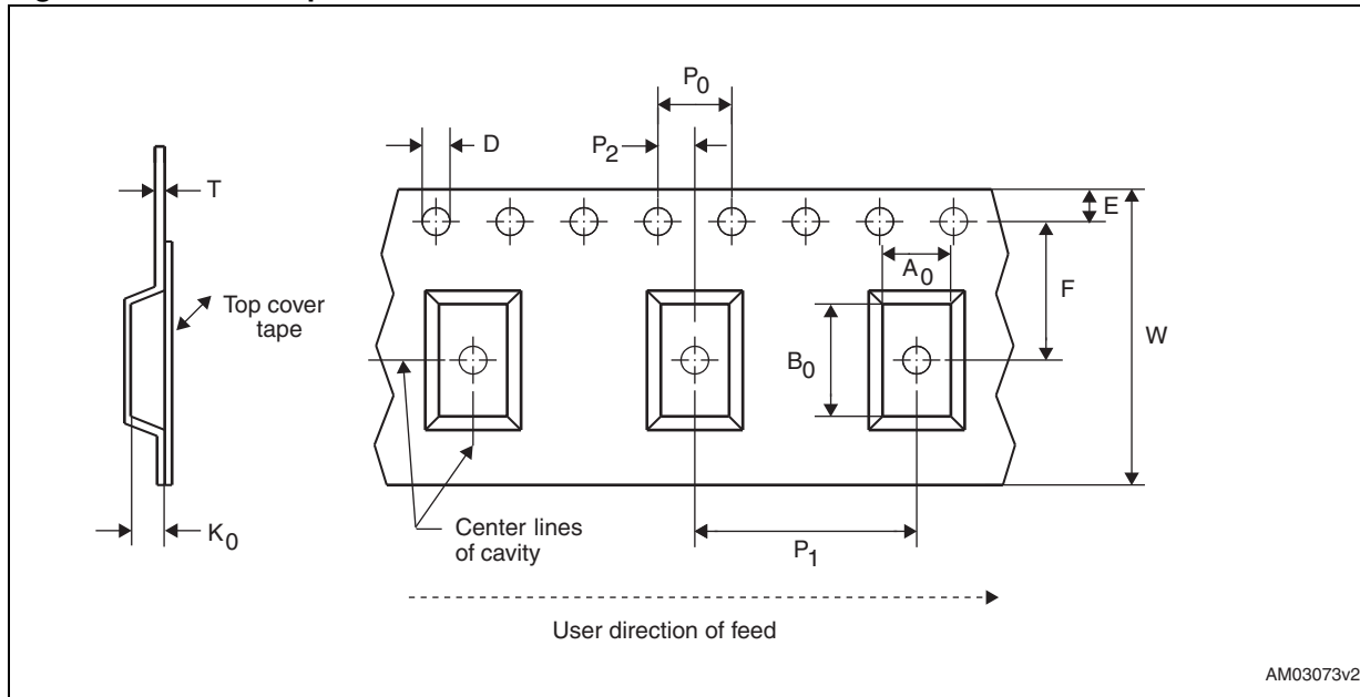
Figure 13. Carrier tape
