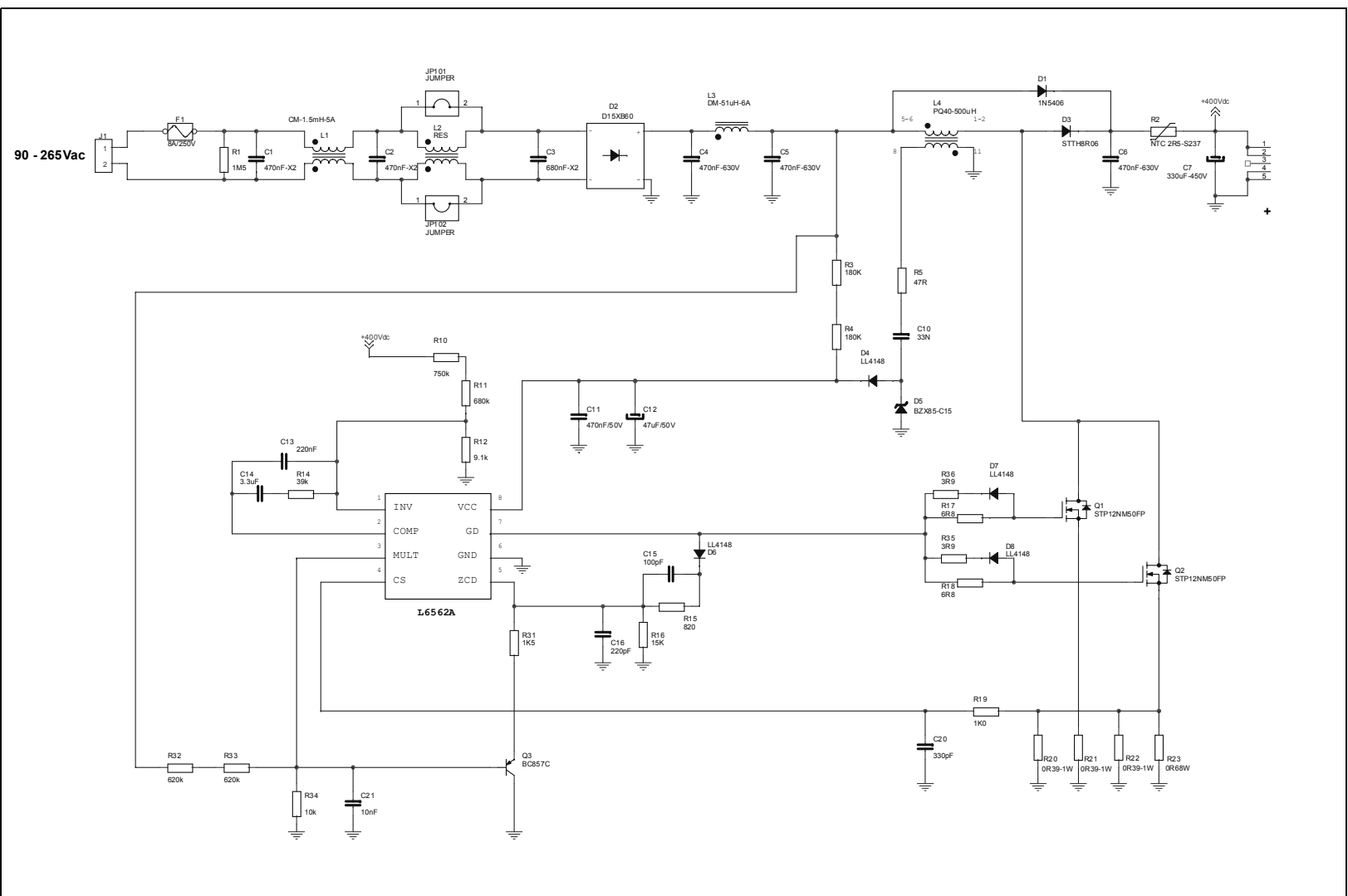
Figure 30. Demonstration board EVL6562A-400W, wide-range mains, FOT
