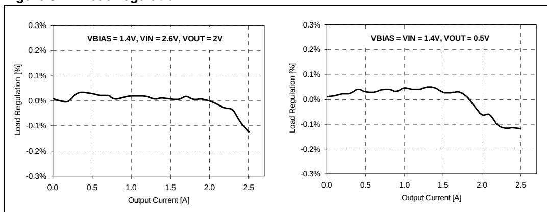
Figure 8. Load regulation
