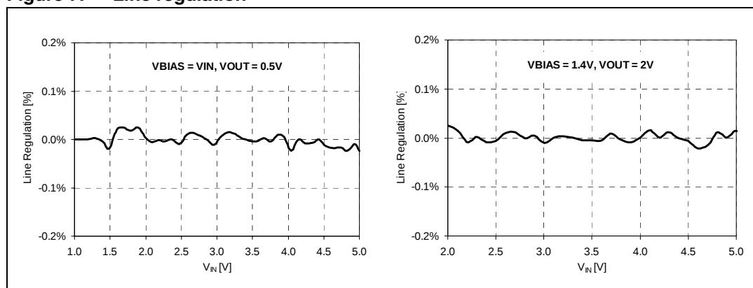
Figure 7. Line regulation
