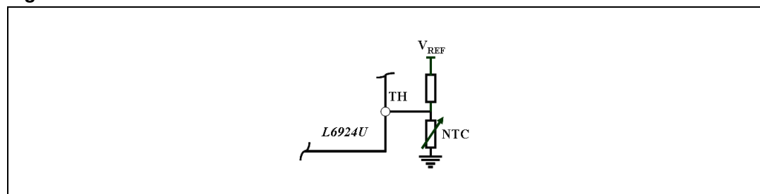
Figure 19. Pin connection
