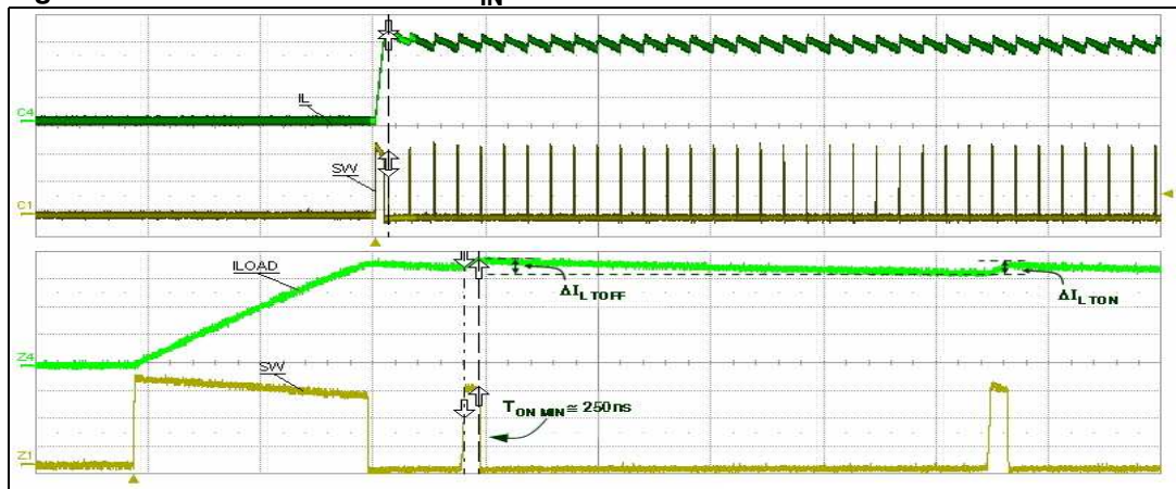
Figure 15. Short-circuit current V_{IN} = 12\ V
