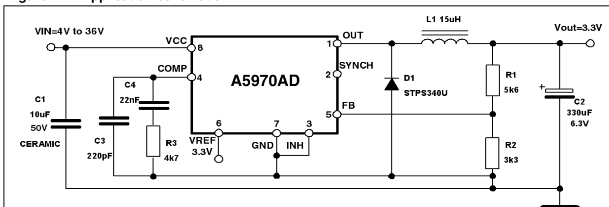
Figure 1. Application schematic
