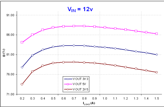
Figure 33. Efficiency vs output current
