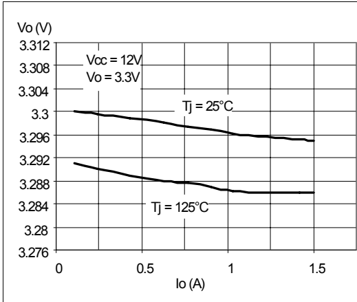
Figure 29. Load regulation
