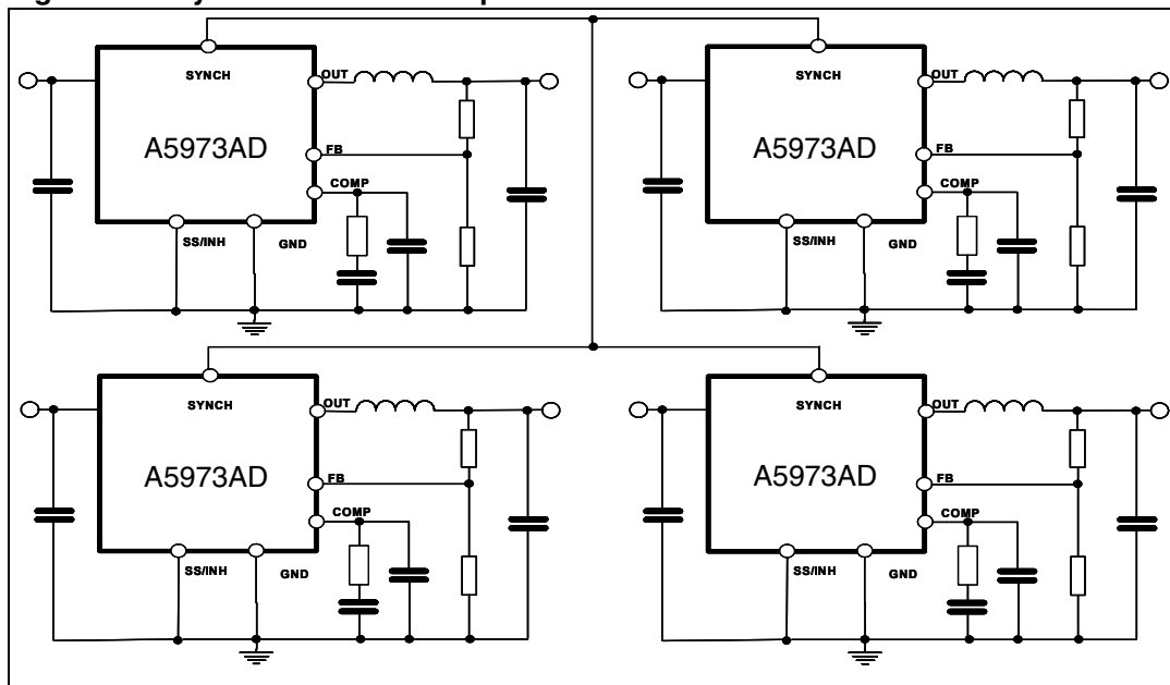
Figure 6. Synchronization example
