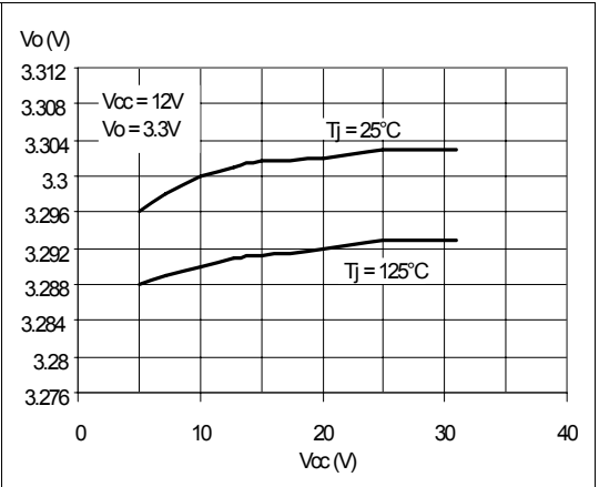
Figure 30. Line regulation
