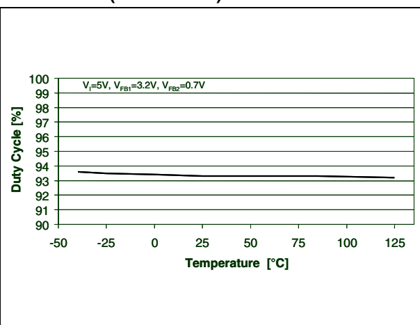
Figure 8. Duty cycle vs. temperature (ST2S06A33)
