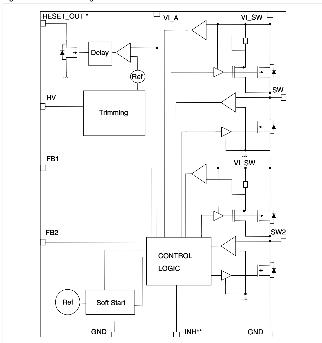
Figure 1. Schematic diagram
