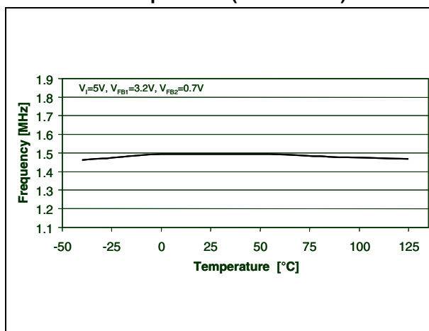
Figure 7. Switching frequency vs. temperature (ST2S06A33)
