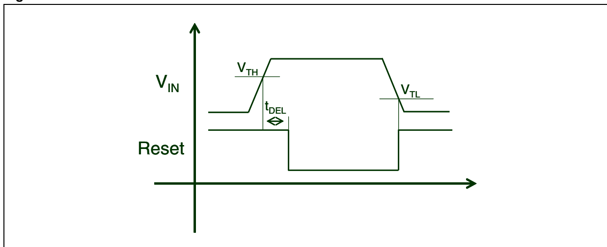
Figure 23. Reset function
