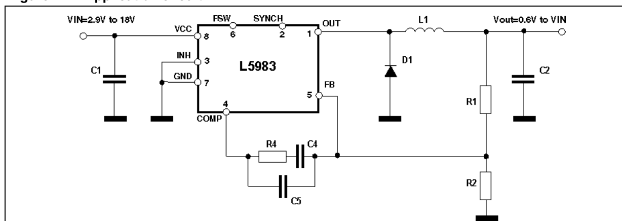
Figure 1. Application circuit
