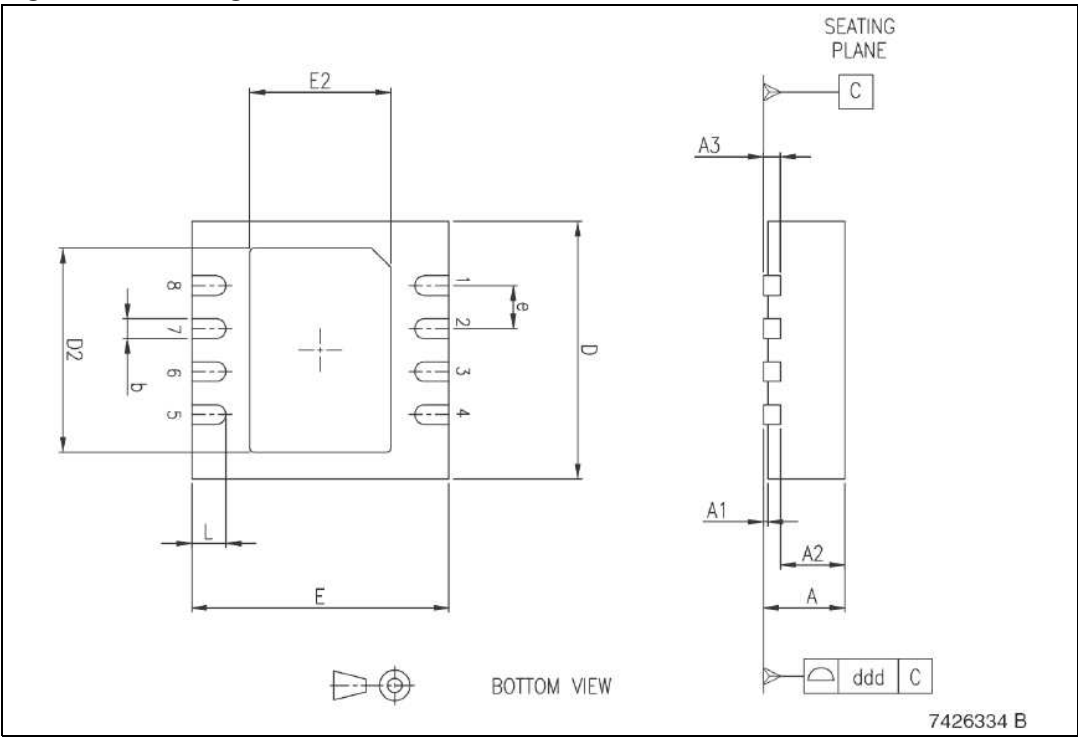
Figure 37. Package dimensions
