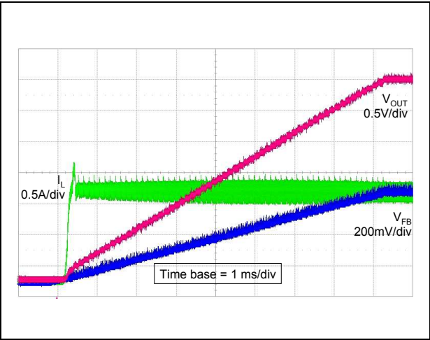
Figure 31. Soft-start
