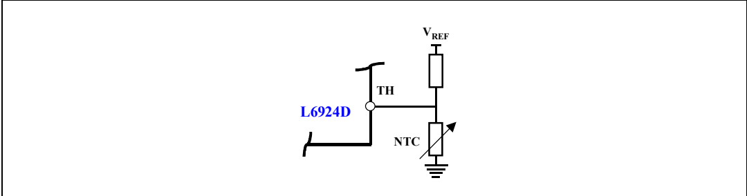
Figure 21. Pin connection
