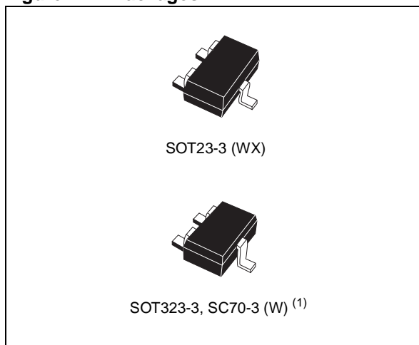
Figure 1. Packages
