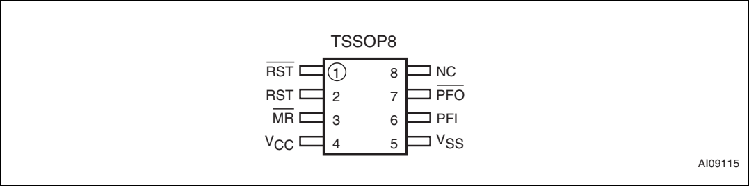
Figure 6. STM707/708 TSSOP8 connections
