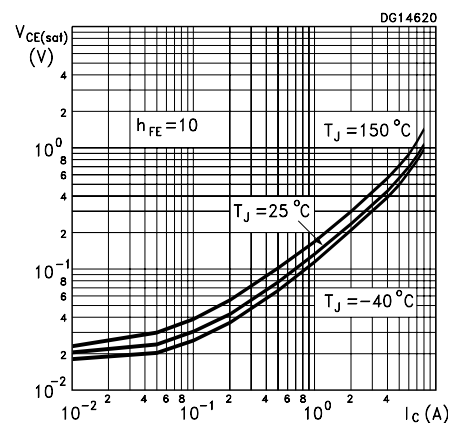
Figure 5. Collector-Emitter Saturation Voltage (NPN)
