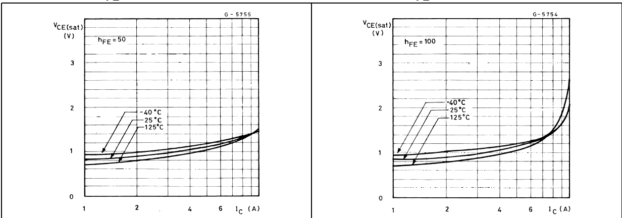
Figure 6. Collector-emitter saturation voltage @ h_{FE} = 50 Figure 7. Collector-emitter saturation voltage @ h_{FE} = 100
