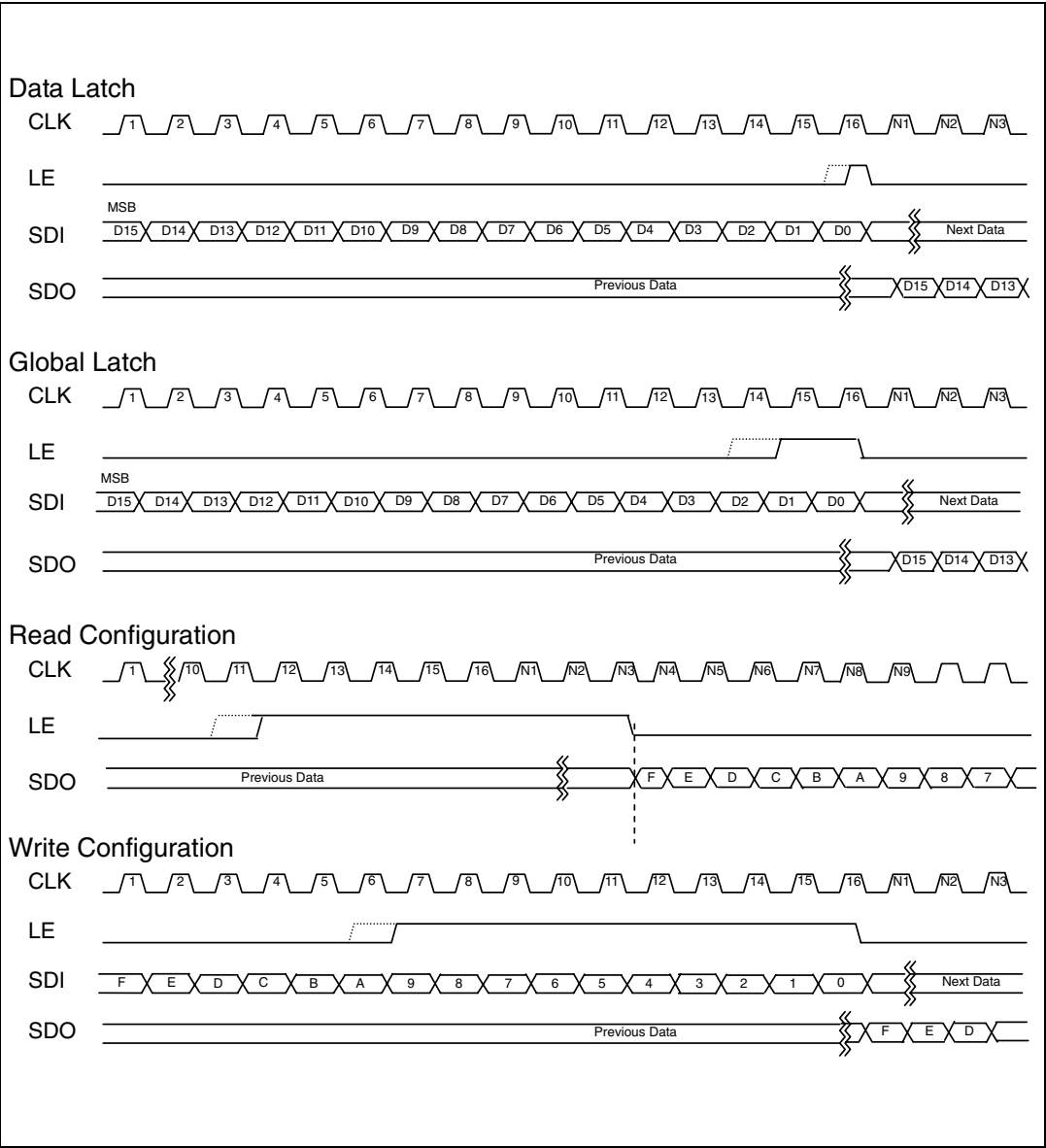
Figure 6. Timing diagram
