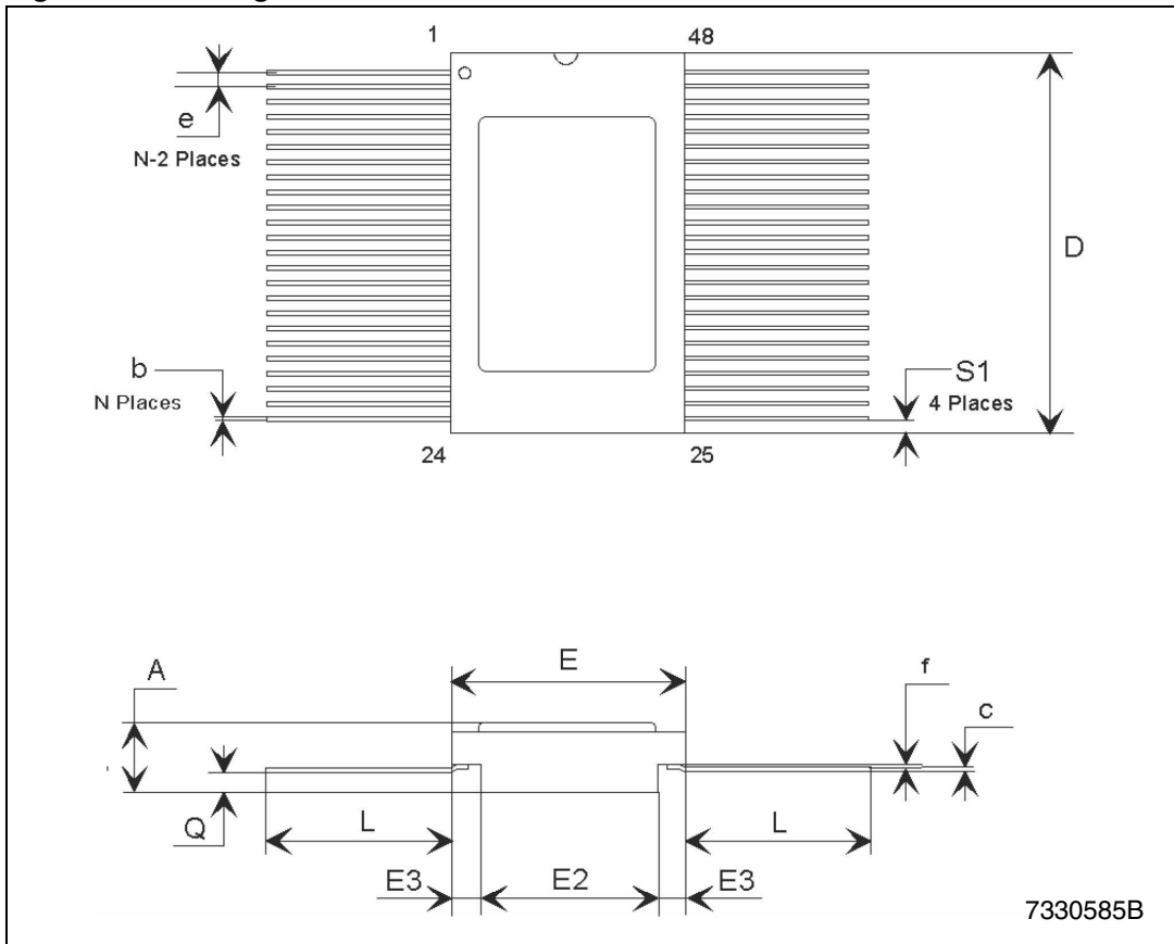
Figure 9. Package dimension
