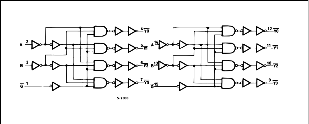
Figure 4. Logic diagram
