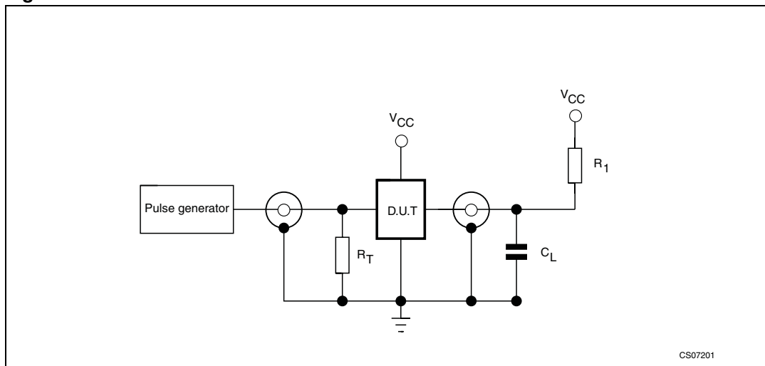
Figure 3. Test circuit
