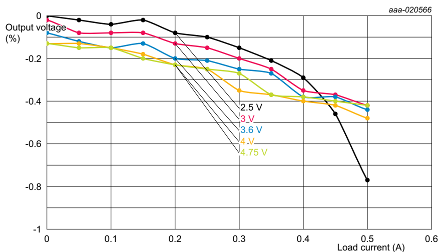
Fig 6. Output regulation vs Iload and V_{IN}
