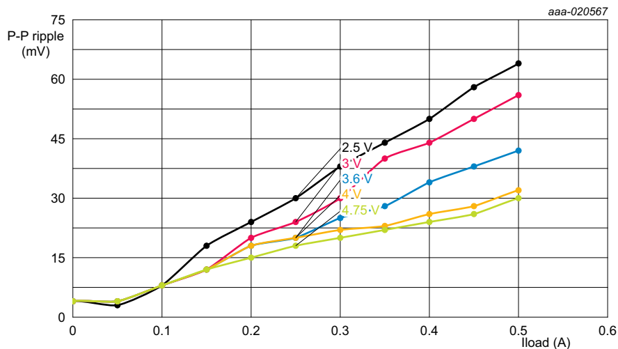
Fig 7. Output ripple vs Iload and V_{IN}
