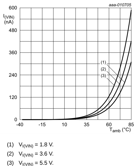
Fig 9. Typical OFF-state leakage current versus temperature
