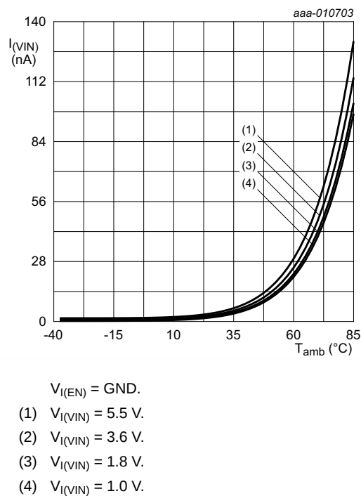
Fig 7. Typical supply current versus temperature
