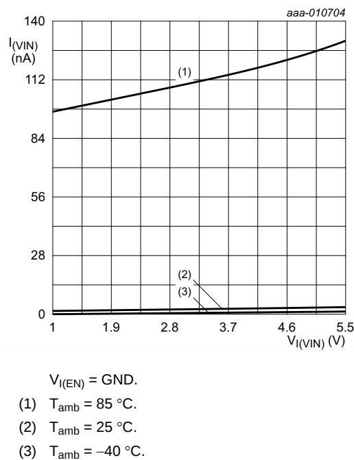
Fig 8. Typical supply current versus input voltage on pin VIN
