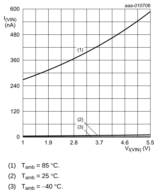
Fig 10. Typical OFF-state leakage current versus input voltage on pin VIN
