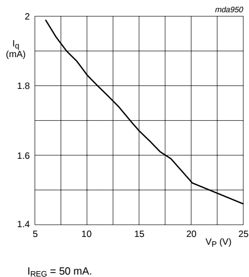
Fig 9. Quiescent current as a function of the supply voltage
