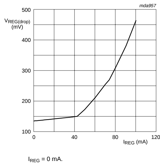
Fig 12. Dropout voltage as a function of the output current
