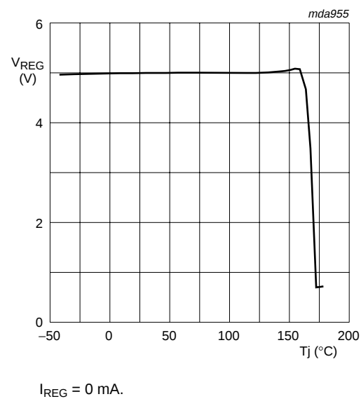
Fig 11. Output voltage thermal protection as a function of the junction temperature
