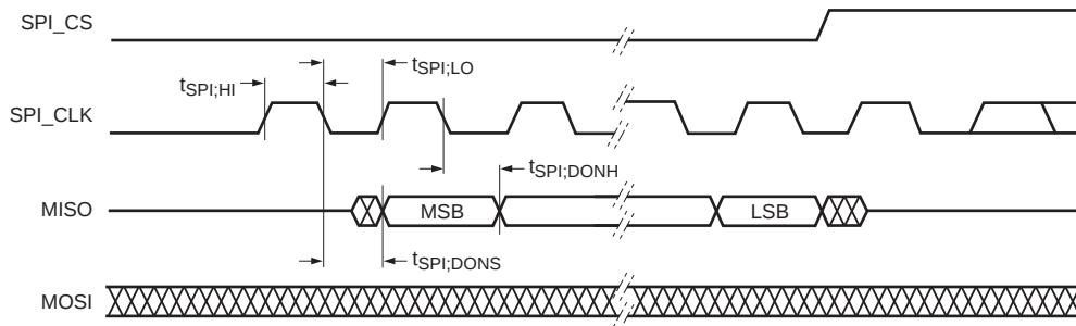
Fig 18. SPI read timing
