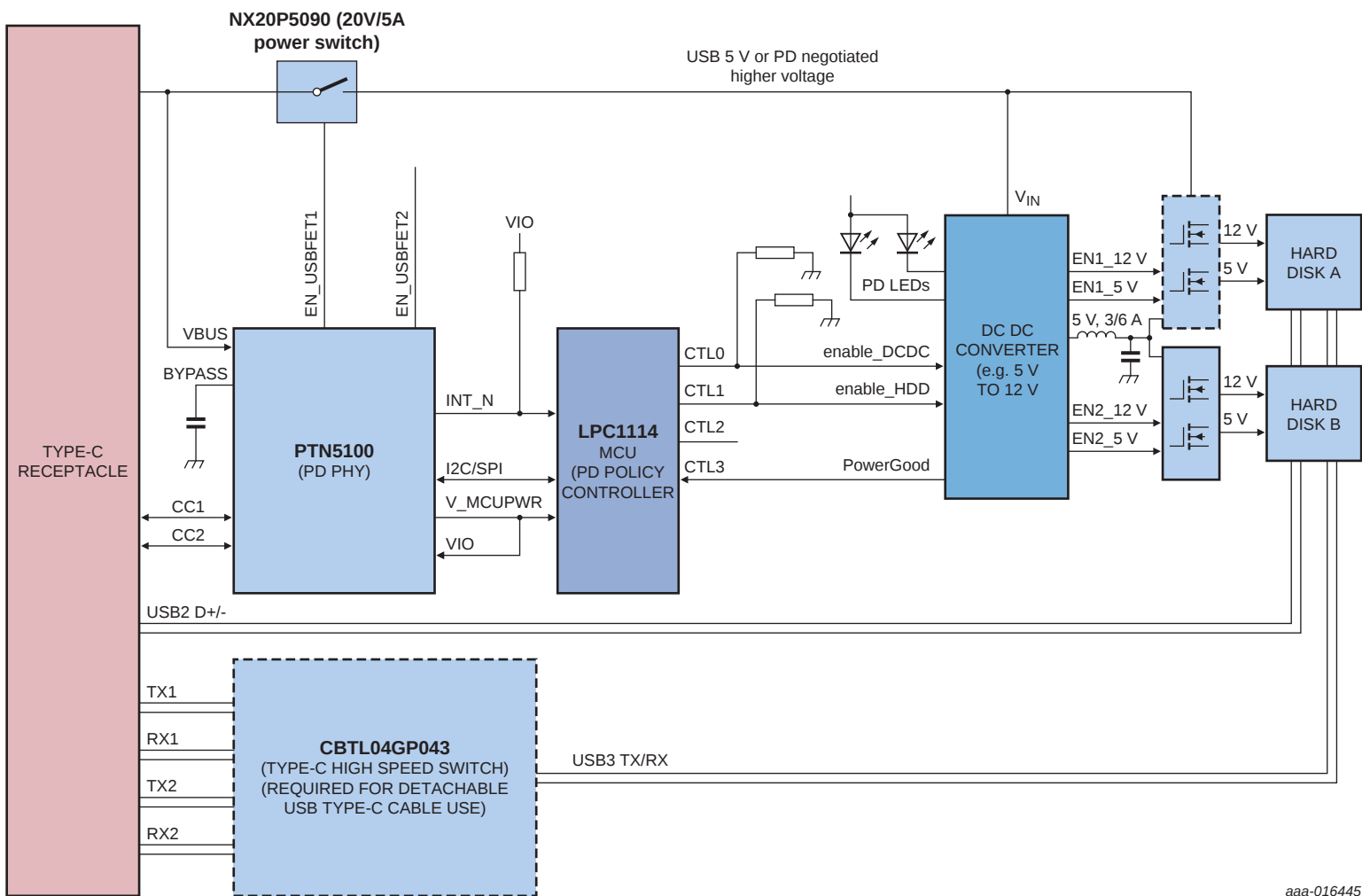
Fig 15. Illustrative diagram of Portable Hard Drive application (sink power path); PD Consumer only
