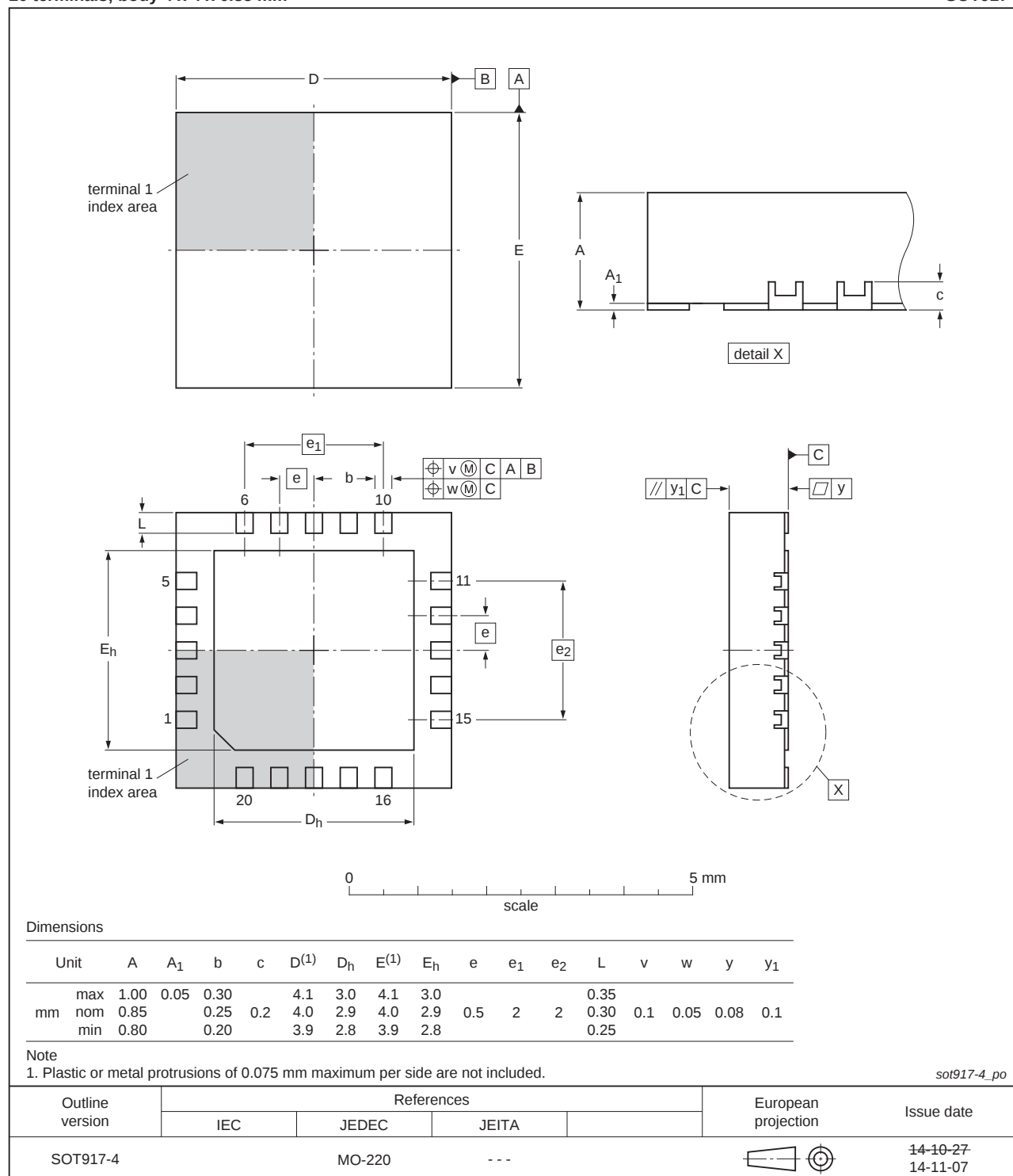
Fig 19. Package outline SOT917-4 (HVQFN20)
