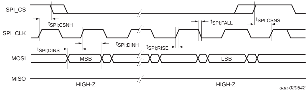
Fig 17. SPI write timing
