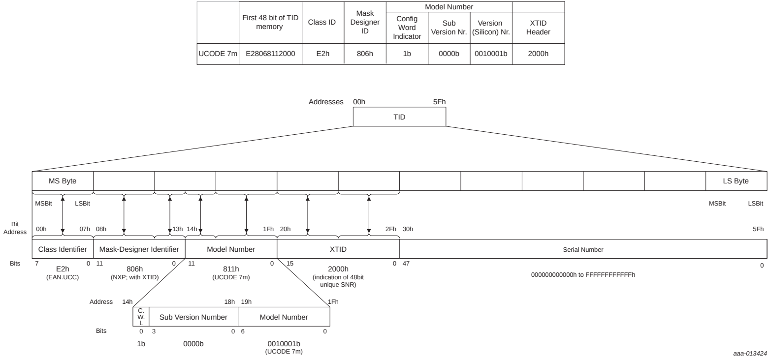
Fig 5. UCODE 7m TID memory structure
