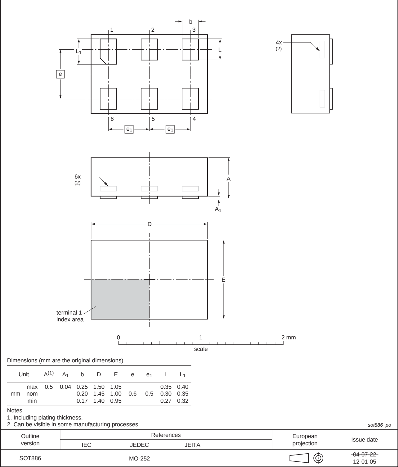
Fig 10. Package outline SOT886
