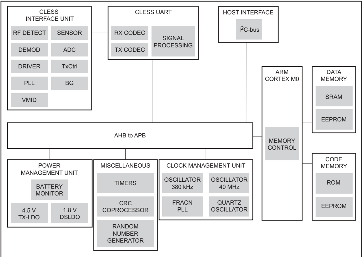
Fig 3. PN7150 block diagram
