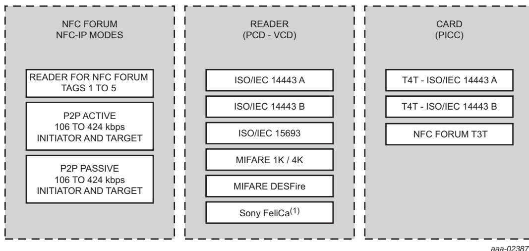
Fig 1. PN7150 transmission modes
