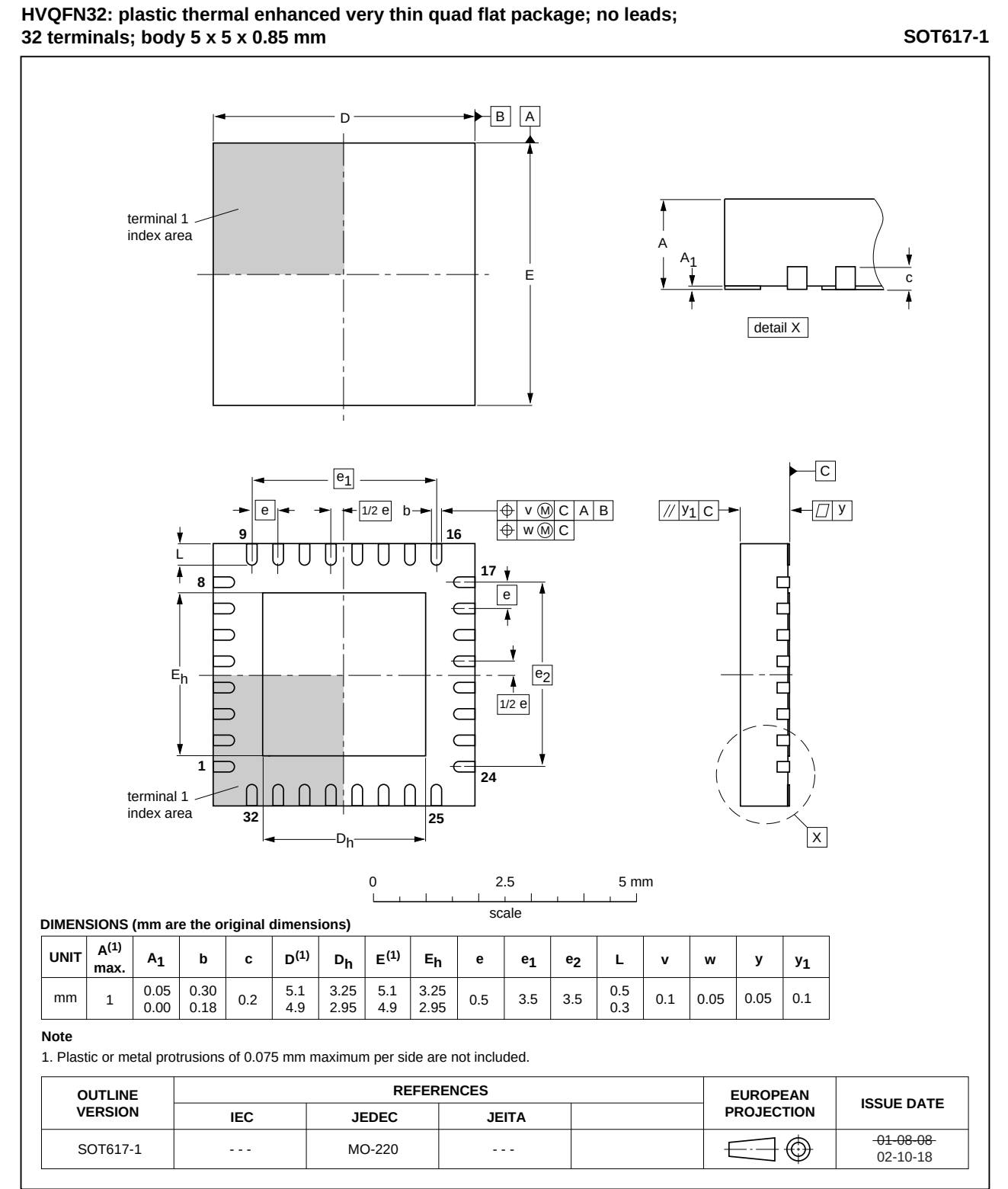
Fig 33. Package outline SOT617-1 (HVQFN32)
