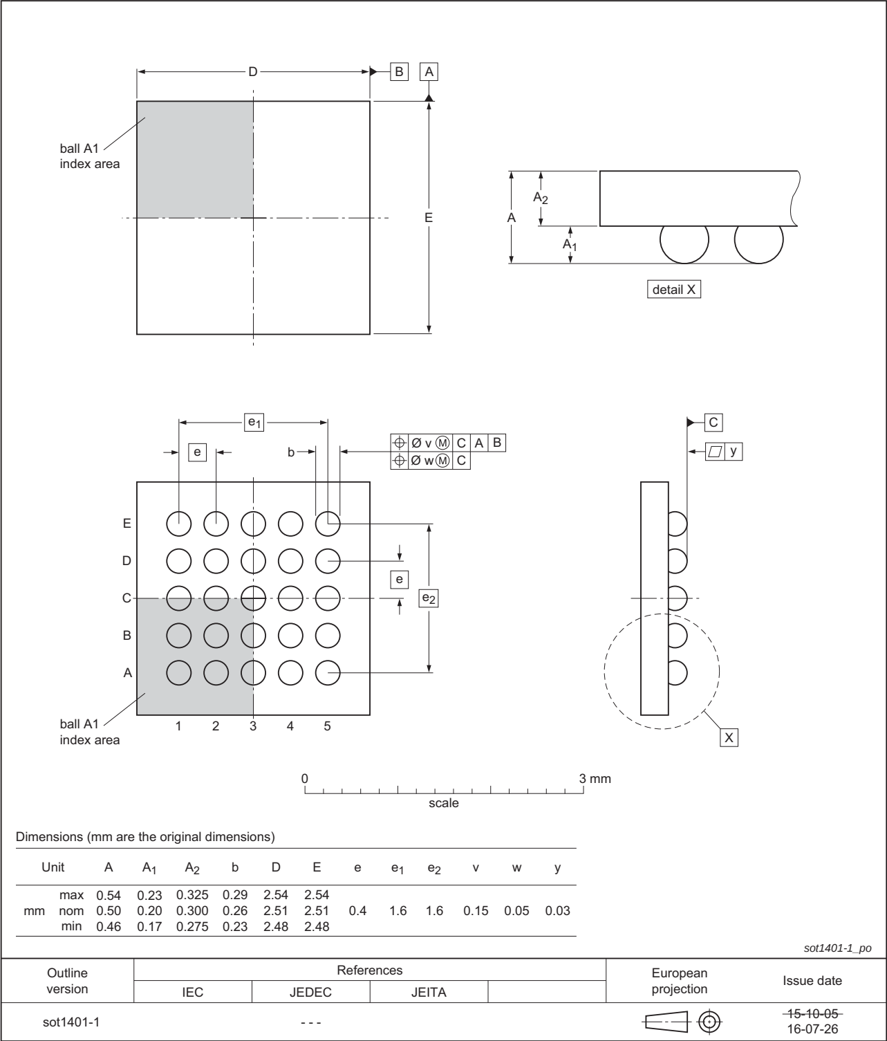
Fig 20. WLCSP25 package outline
