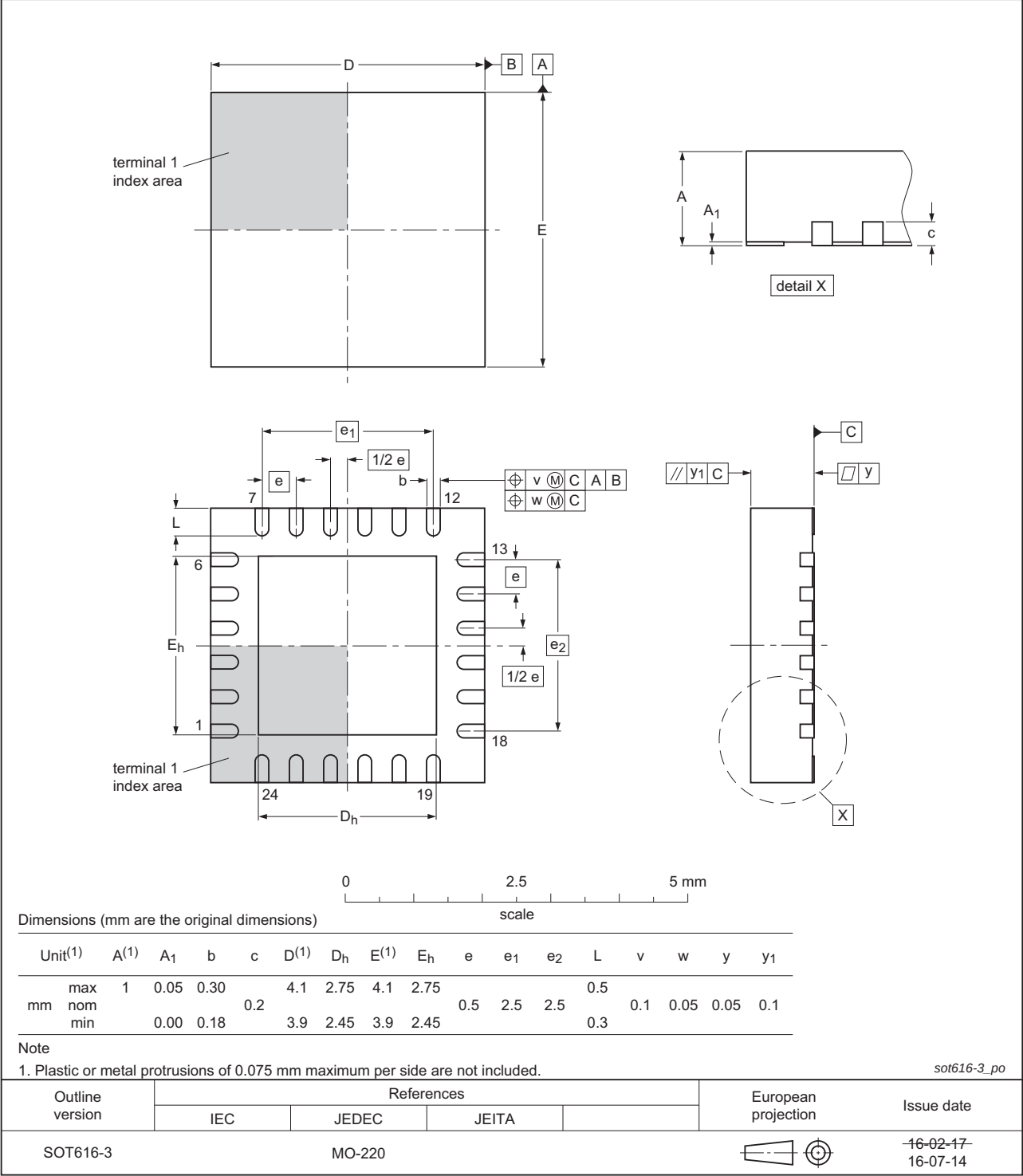
Fig 19. HVQFN24 package outline
