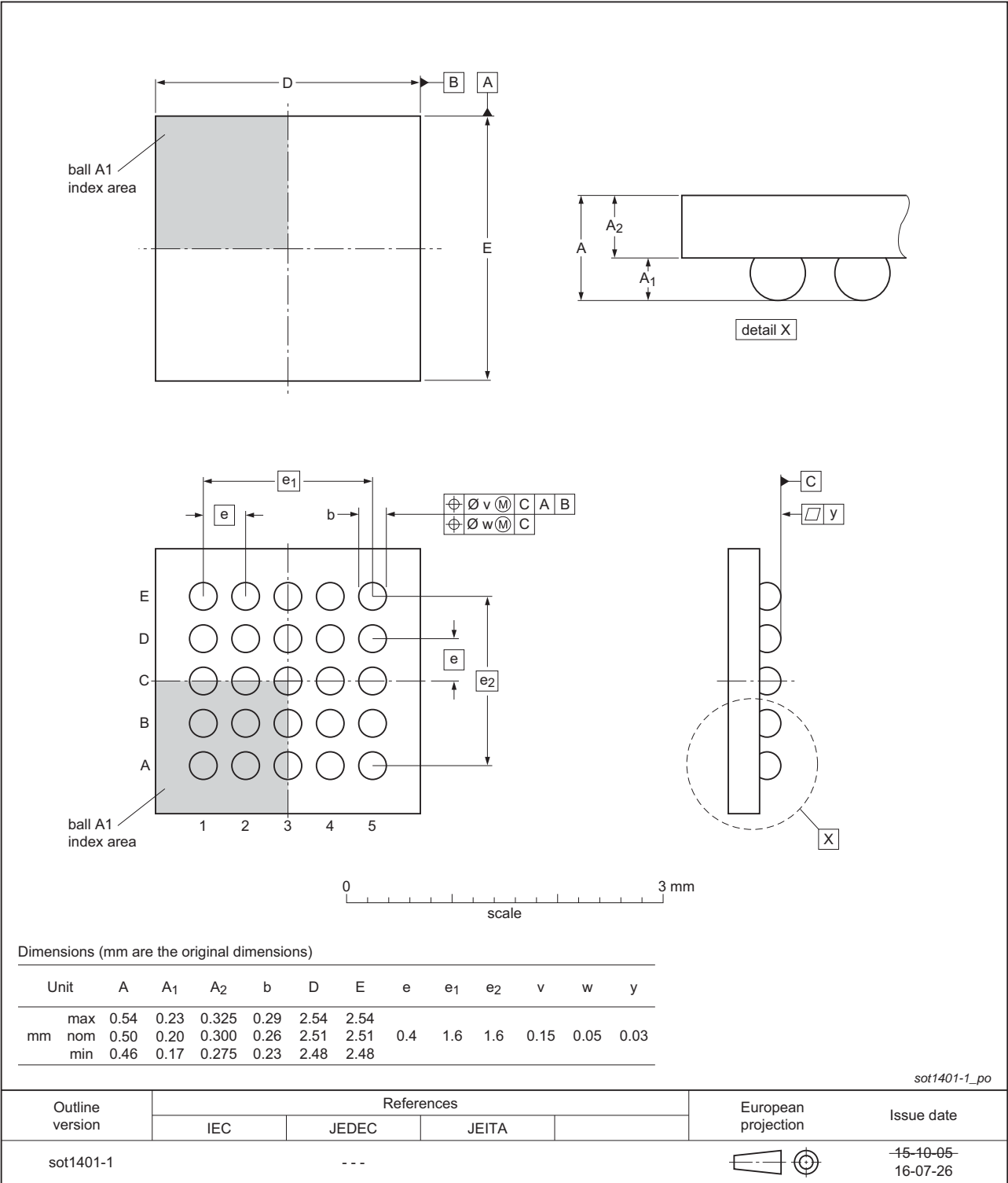
Fig 16. WLCSP25 package outline
